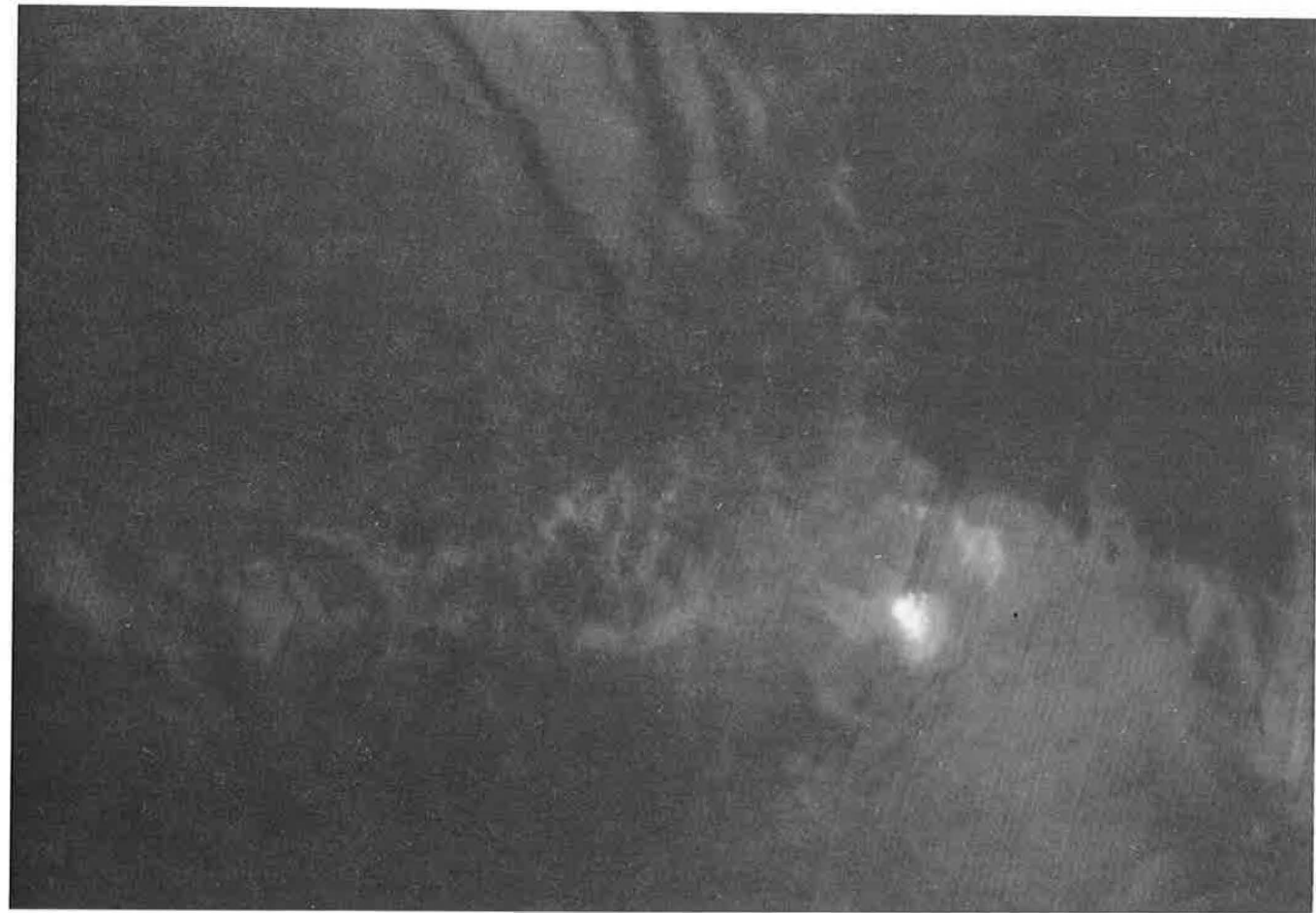
Figure 3. Thermal infrared image of the same area, showing the initial crater, March 27, 4:15 p.m. Numerous fumaroles (gas vents) are clustered along the floor of the crater.
